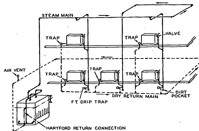
FIG. 11. TYPICAL DOWN-FEED TWO-PIPE SYSTEM
