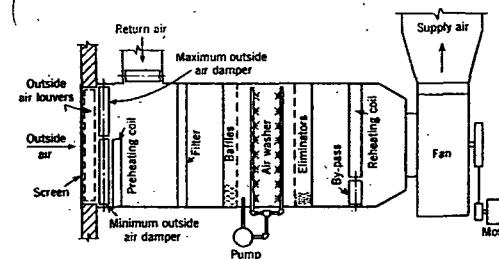
FIG. 1. CENTRAL SYSTEM FOR WINTER AIR CONDITIONING
