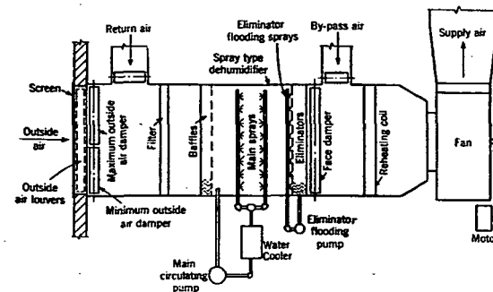
FIG. 3. CENTRAL SYSTEM FOR YEAR 'ROUND AIR CONDITIONING
