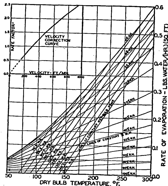
FIG. 8. RATE OF EVAPORATION CHART 3
