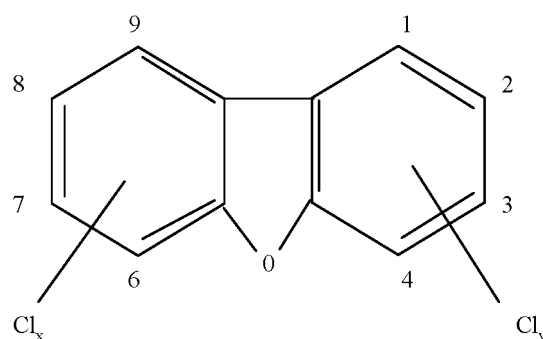
PCDFs
