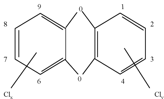
PCDDs
