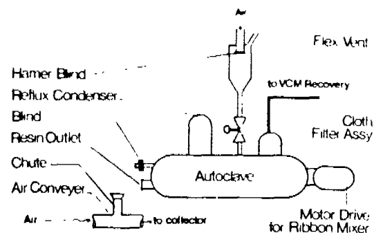
Figure 2 — Bulk process reactor
