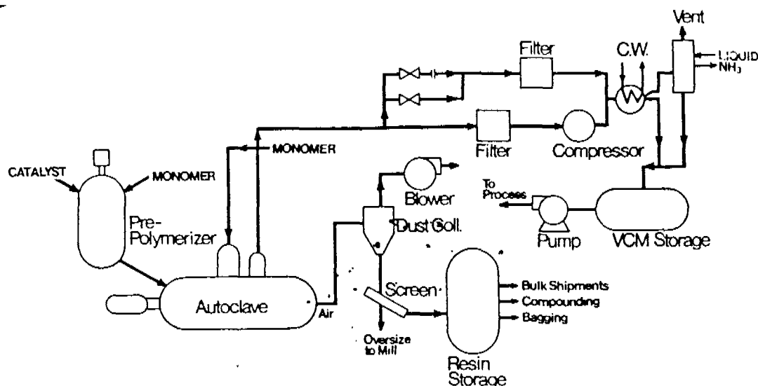
Figure 1 — Bulk polymerization process for polyvinyl chloride
