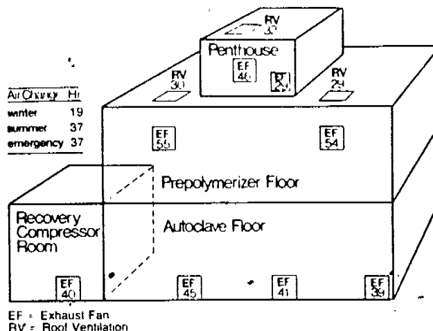
Figure 3 — General ventilation system
