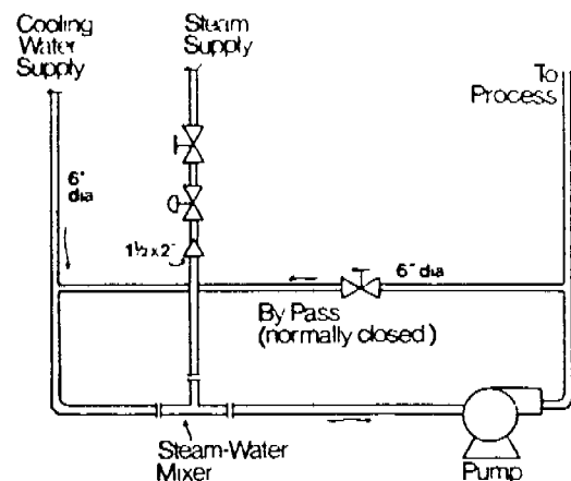
Figure 5 — Steam-water mixer.
