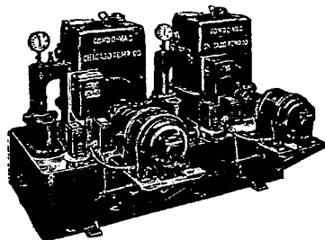
Fig. 2102—Duplex "Condo-Vacs" with Duplex Double Automatic Control
