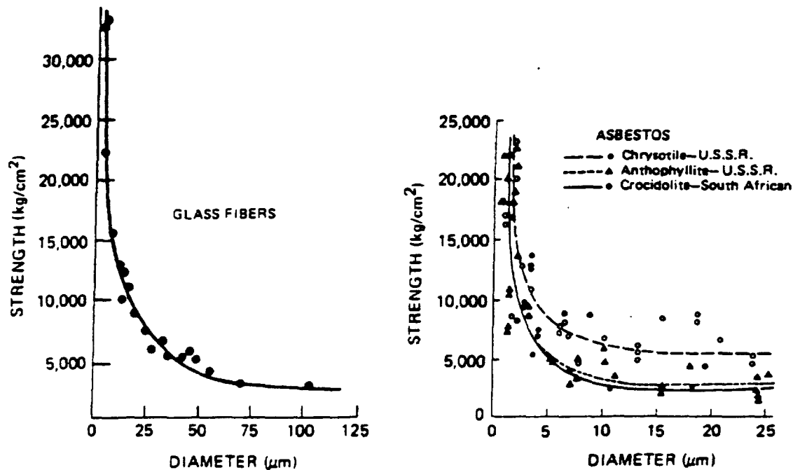
FIGURE 2-4. Illustration of the strength-diameter effect. Data from Griffith, 1921 (glass fibers) and Nadgornyi et al. , 1965 (asbestos).
