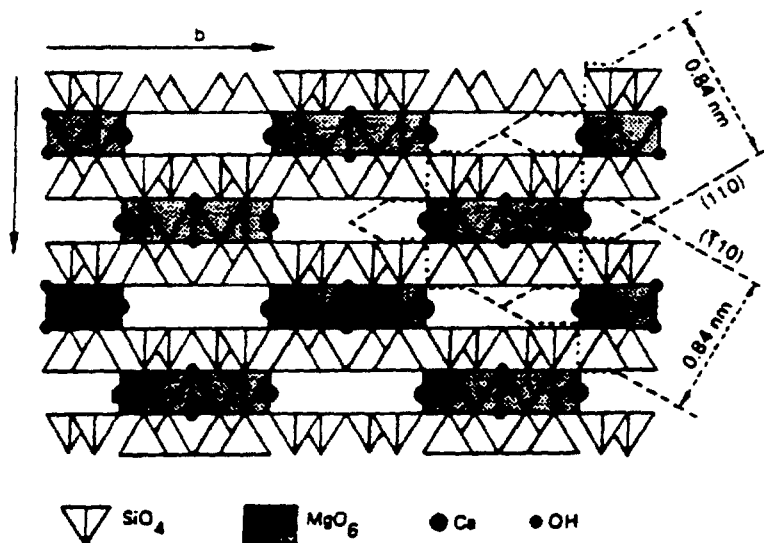
FIGURE 2-3. Diagram of the structure and cleavage of amphibole crystals. Because of structural weakness, the crystal preferentially breaks along the (110) and (110) planes, parallel with the c-axis, yielding acicular fragments. From Zoltai, 1979.
