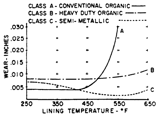
Fig. 3-Average wear versus temperature characteristics, inertia dynamometer, 1740 lb wheel load, ventilated rotor
