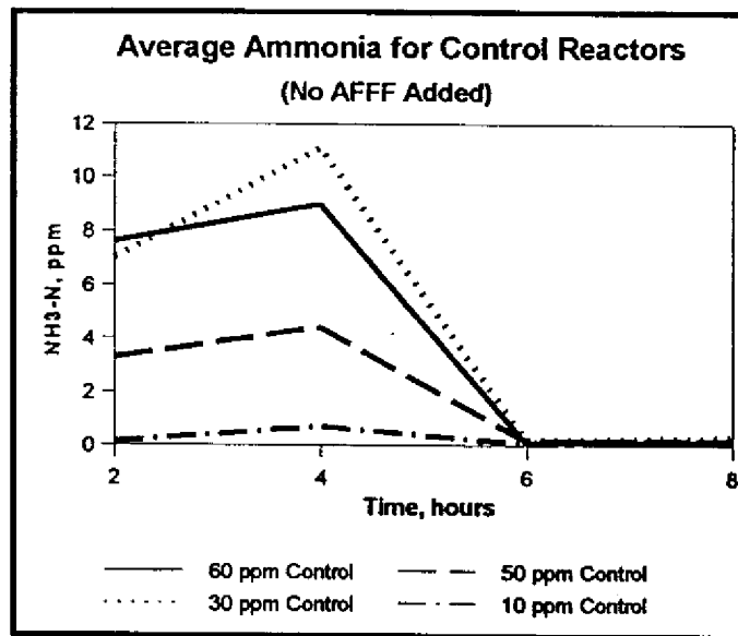
Figure 4-2a. Average Ammonia Concentrations for Control Reactors
