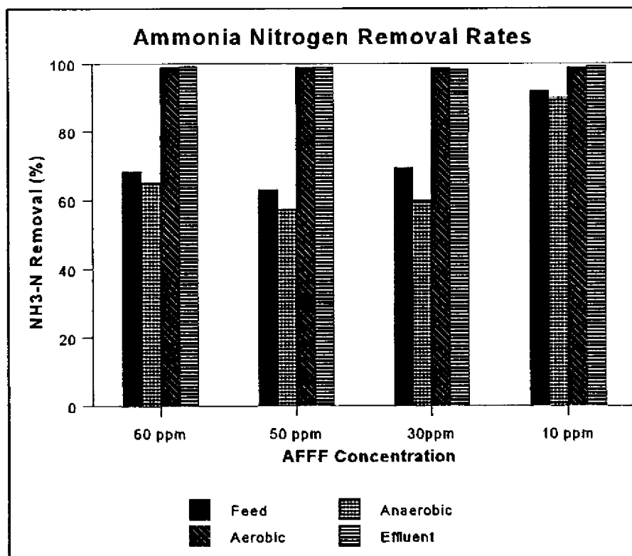
Figure 4-3. Average Ammonia Nitrogen Removal Rates for the Inhibition Reactors
