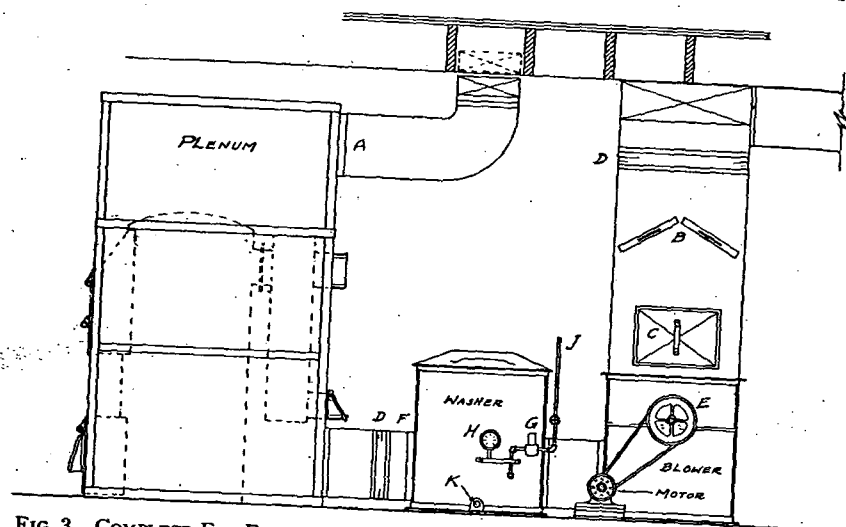
FIG. 3. COMPLETE FAN FURNACE INSTALLATION SHOWING LOCATION OF FAN, FURNACE, FILTERS, PLENUM CHAMBER AND METHOD OF TAKE-OFF OF WARM AIR PIPE
