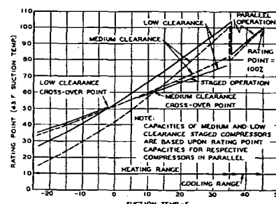
Fig. 8.... Comparison of Parallel and Staged Operation
