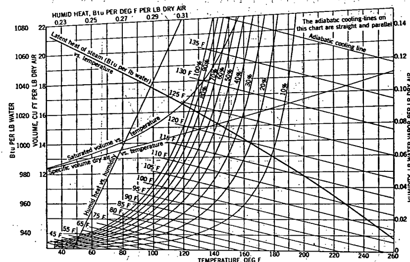
FIG. 6. PSYCHROMETRIC CHART
