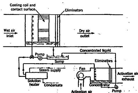
FIG. 5. LIQUID-ABSORBENT EQUIPMENT IN WHICH SOLUTION COOLER AND CONTACTOR ARE COMBINED
