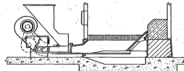
FIG. 4. UNDERFEED SIDE CLEANING STOKER
