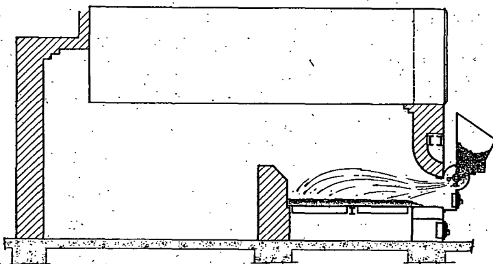
FIG. 3. OVERFEED SPREADER STOKER, ROTOR TYPE
