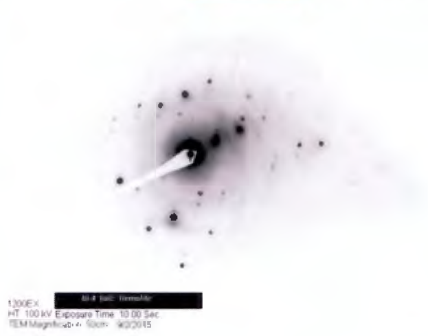
FIGURE 4 Selected-area electron diffraction (SAED) of tremolite structure found in the Indian talc product "ID.4 Talc." All asbestos structures used in the calculation of concentrations in this report were confirmed by morphology, chemistry (by energy-dispersive X-ray analysis: EDXA/EDS), and crystalline structure as demonstrated here by diffraction (SAED). Notice the 5.3 Å repeat of streaking lines consistent with the amphibole structure, and the arcing brighter bands demonstrating a nearby crystal zone axis
