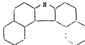
3,4,5,6-dibenzcarbazole
