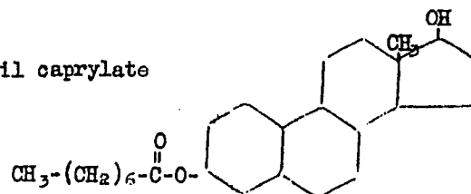
1,2-cyclopentone phenanthrene 2
