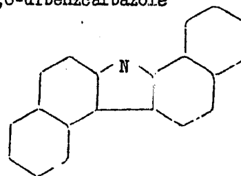
1,2,5,6-dibenzcarbazole
