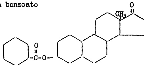
Equilenin benzoate
