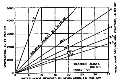
(Vapor Barrier, 1 perme Wall and Ceiling Area 2000 sq ft Insulated)
