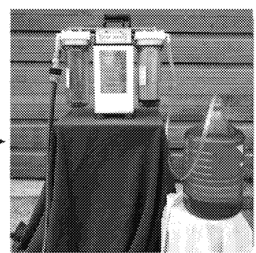
2. Pressurized Water Input Via Garden Hose Collected At Output
