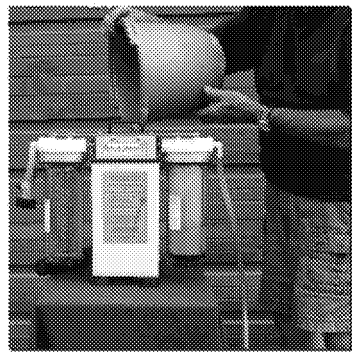
4. Fill Holding Tank With Water From Pond, Lake, Stream, Etc.
