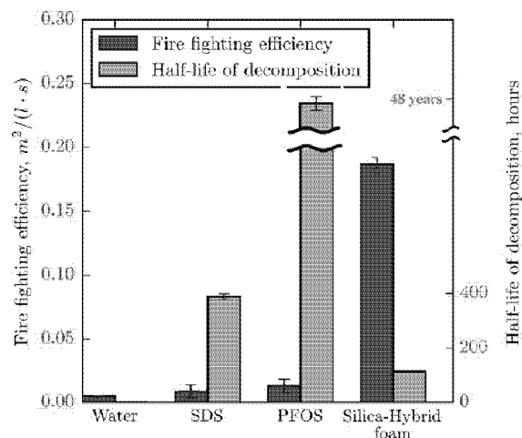
Figure 8. Comparison of fire-fighting efficiency and biodecomposition properties for agents used in extinguishing solid combustibles.
