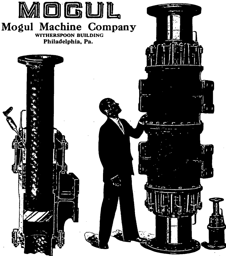
"MOGUL" DOUBLE-END-GUIDED, TYPE F. L. J. (FLANGED) EXPANSION JOINTS
