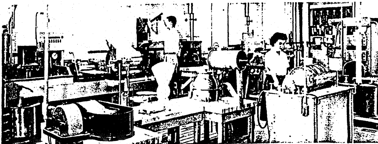
To aid in the development of improved pigments for the paper industry, the complete paper-making process can be duplicated in this section of the new Chemicals Division laboratory.
