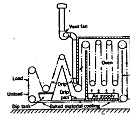
FIG. 5. SMALL PART MULTIPLE PASS OVEN FIG. 6. INCLINED END ENAMELING OVEN
