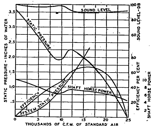
FIG. 2. SOUND LEVEL CHARACTERISTICS OF TYPICAL VANEAXIAL FAN
