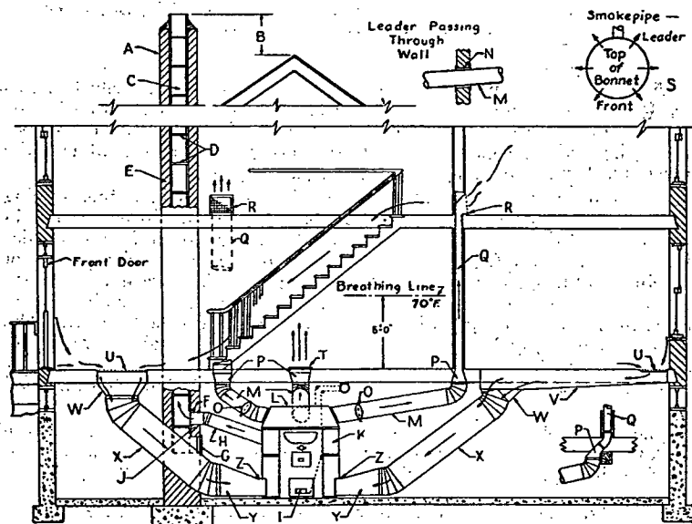
FIG. 1. A SECTIONAL VIEW OF A TYPICAL PLANT SHOWING GOOD INSTALLATION PRACTICE*
