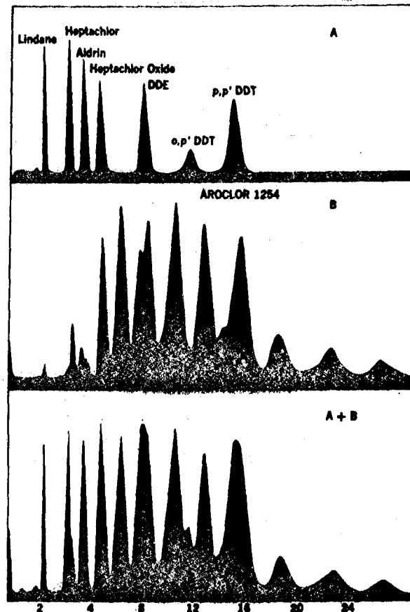
Gas chromatogram A is of a standard pesticide mixture, B is typical of Aroclor 1254, and A + B is the chromatogram of a 50:50 mixture of both. The concentration of Aroclor 1254 is approximately 10 times those of the pesticides in A, hence it is understandable why PCB's were not readily recognized in pesticide chromatograms. Gas chromatograph (Packard 7620) conditions: gas flow 80 ml./min. nitrogen, temperatures—oven, 210° C.; inlet, 230° C.; detector, 218° C.; N 2 electron capture detector; B' x 1/4" glass column packed with 8% SE-30 on Chromosorb Q 80-80 mesh.
