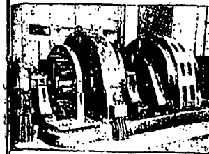
1100 KW General Electric 3 Unit - 3 Bearing Motor Generator set taken on foundation. Now on our shop floor available for immediate shipment as it is built. Generator 1500 KW - type MT-45Y - 600 volts; Motor 1100 HP - 7 ph - type AT1 2200/4130 volt - 3 ph. 60 cy.
