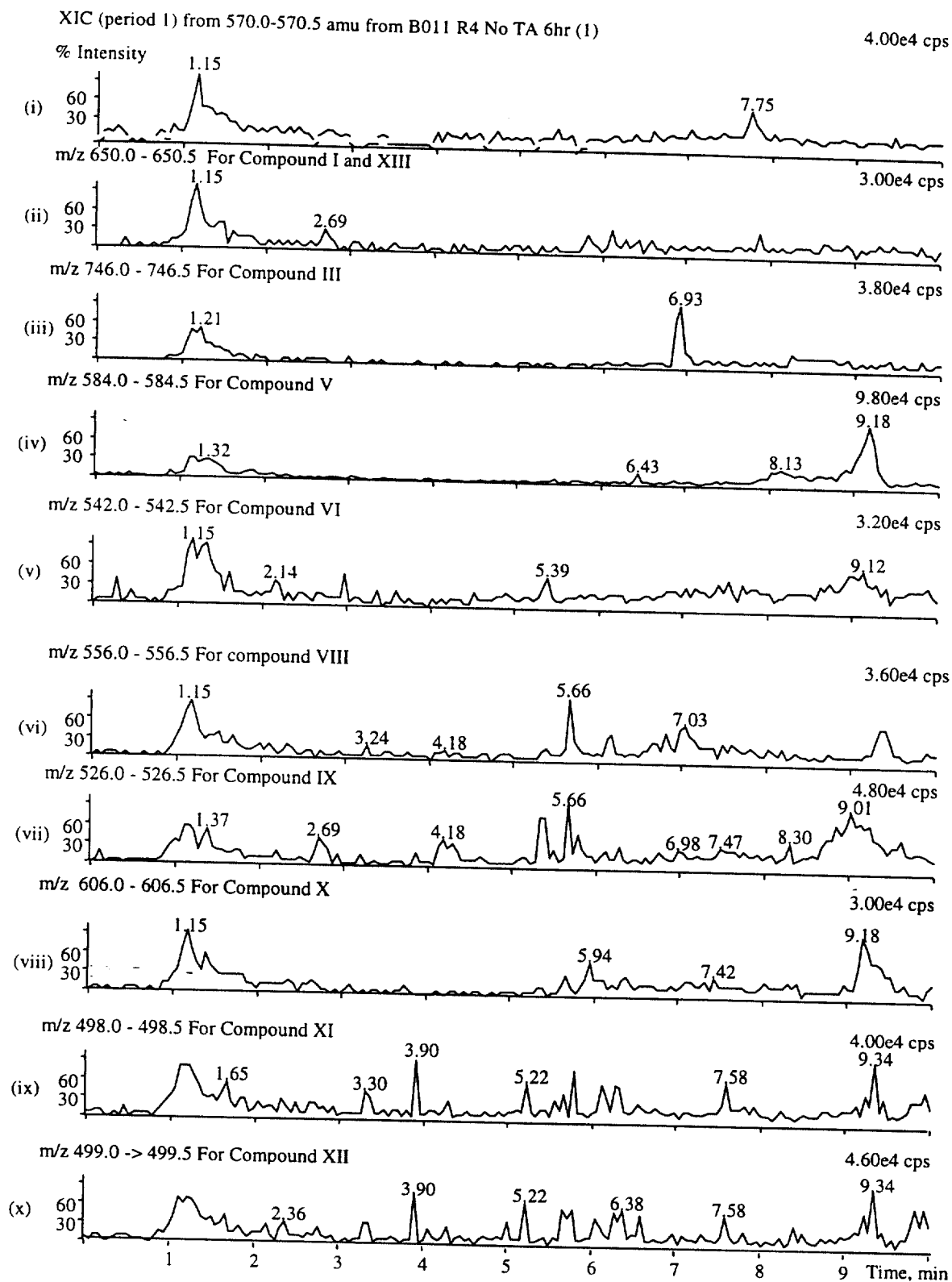
Figure 4. Full scan reconstructed ion chromatograms of control rat hepatocytes incubated for 6 hours with no test articles
