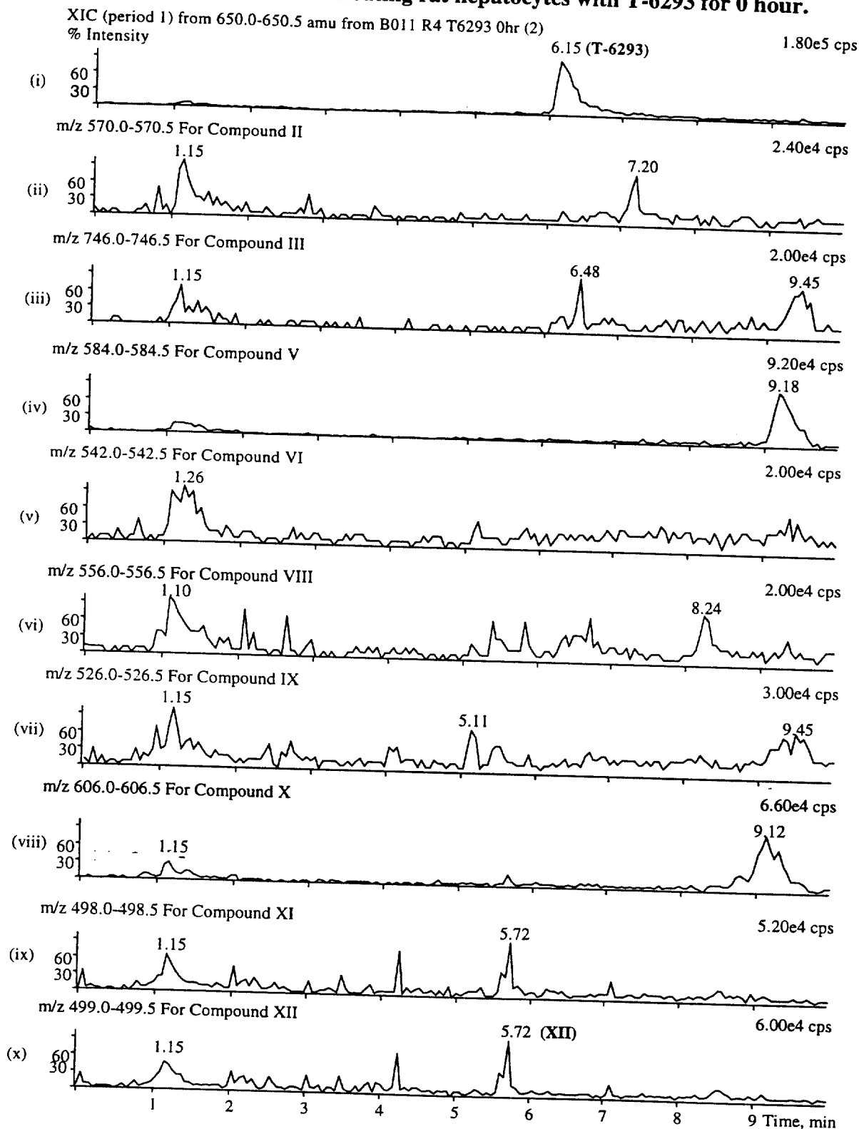
Figure 18. Full scan reconstructed ion chromatograms showing the presence of metabolites after incubating rat hepatocytes with T-6293 for 0 hour.
