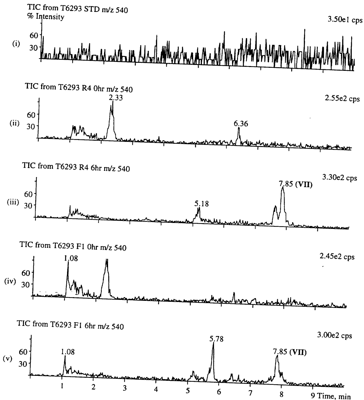
Figure 23. SRM total ion chromatograms showing the presence of metabolite VII in (i) T-6293 standard solution; (ii) incubation of T-6293 with rat hepatocytes at 0 hour; (iii) incubation of T-6293 with rat hepatocytes at 6 hour; (iv) incubation of T-6293 with human hepatocytes at 0 hour and (v) incubation of T-6293 with human hepatocytes at 6 hour.
