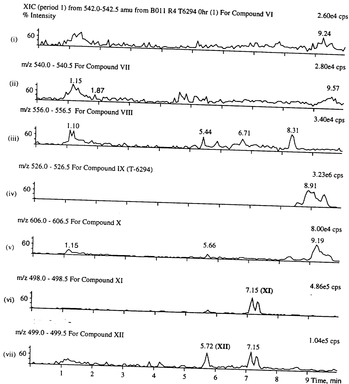
Figure 26. Reconstructed ion chromatograms showing the presence of metabolites after incubating rat hepatocytes with T-6294 for 0 hour.
