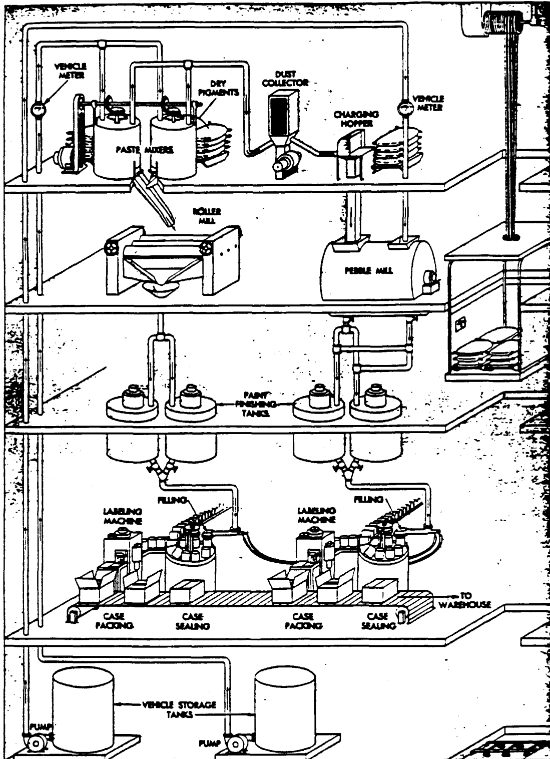
PAINT PLANT FLOW CHART
