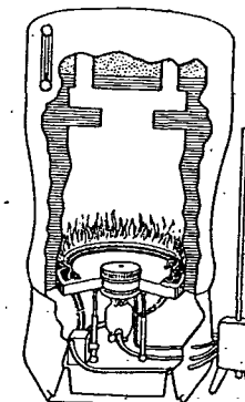
FIG. 14. WALL FLAME VERTICAL ROTARY BURNER
