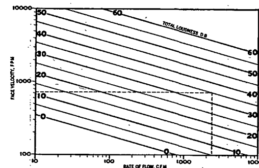
FIG. 5. AIR FLOW AND LOUDNESS CHART
