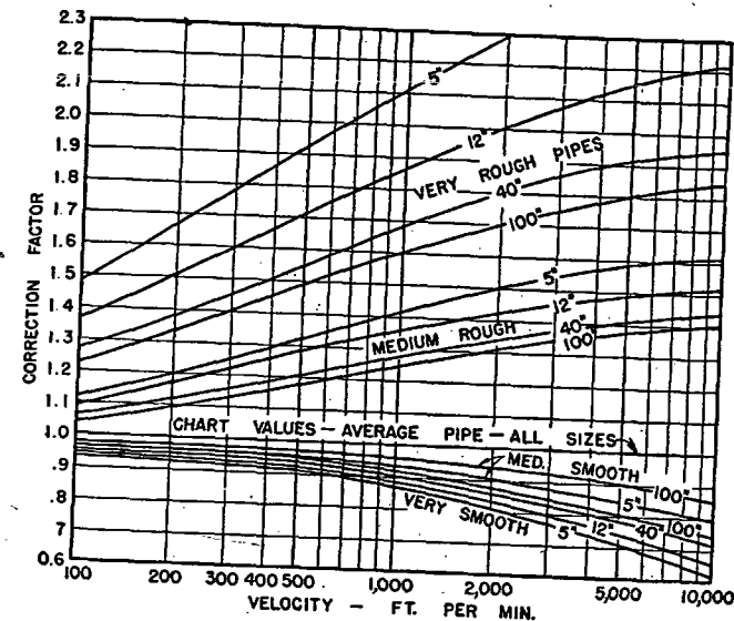
FIG. 3. CORRECTION FACTORS FOR PIPE ROUGHNESS
