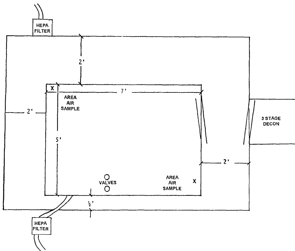
FIGURE 2. Diagram of enclosure for valve packing removal study.
