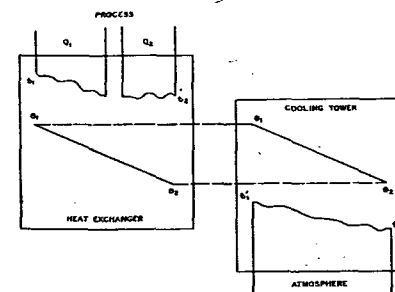
Fig. 9.... Relation of Cooling Tower to Process
