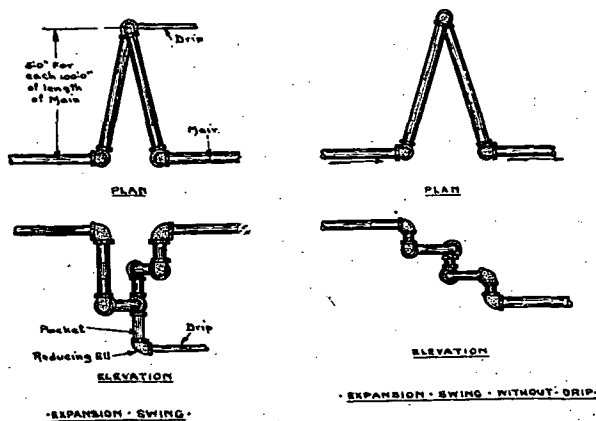
FIG. 23. TYPICAL EXPANSION CONNECTIONS FOR RISERS
