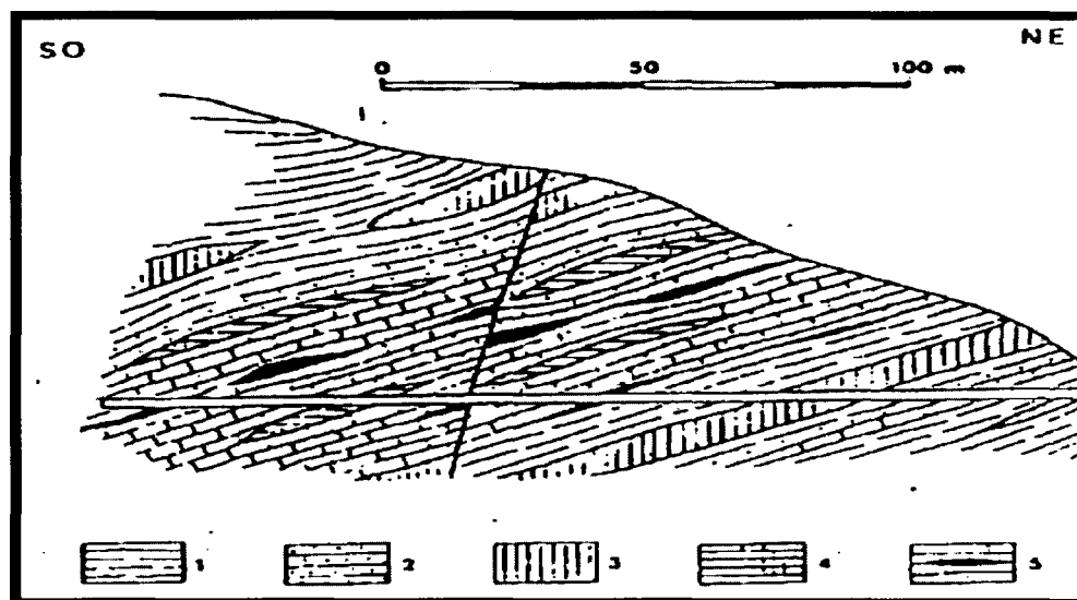
Fig. 3 - Structure of the of dolomitic limestone bank mineralized with talc in the Ribasso Cevrero from the former Martinetto mine in Sangone Valley.
