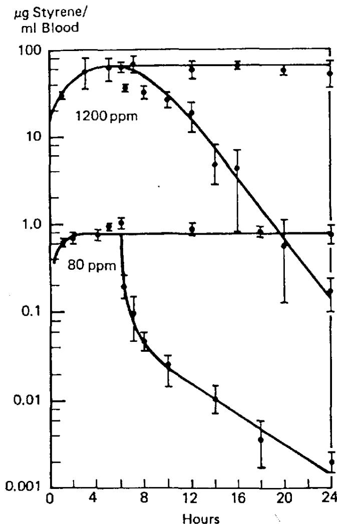
FIGURE 2. Blood styrene concentration in humans exposed to 80 ppm for 6 hr. Data from Ramsey and Young (23).
