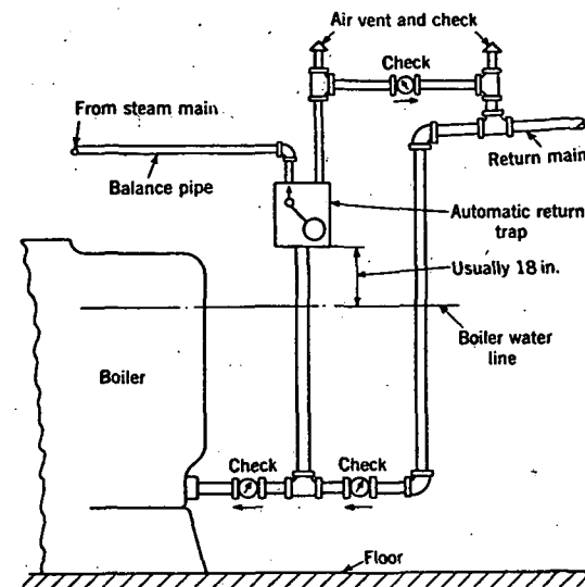
FIG. 9. TYPICAL CONNECTIONS FOR AUTOMATIC RETURN TRAP
