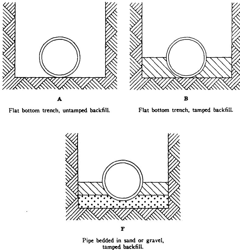
Fig. 1. Laying Conditions for Gray Cast-Iron Pipe
