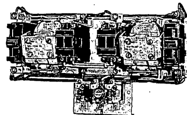
Size 2 — Horizontal Construction 3 Coil Overload Relay
