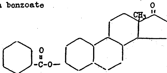
Equilenin benzoate
