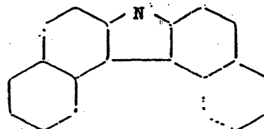
3,4,5,6-dibenzcarbazole
