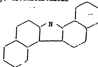
1,2,5,6-dibenzcarbazole
