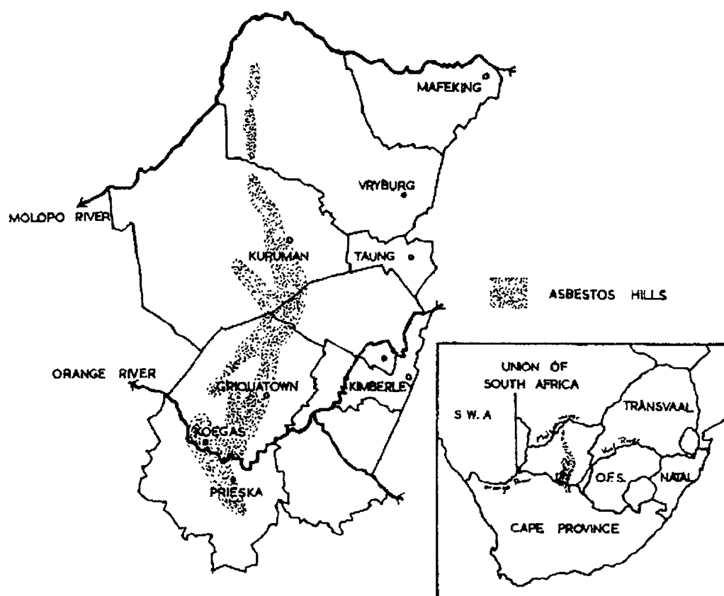
FIG. 1.—Map of Griqualand West asbestos fields.
