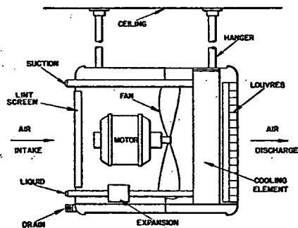
FIG. 3. SUSPENDED PROPELLER FAN TYPE UNIT AIR CONDITIONER
