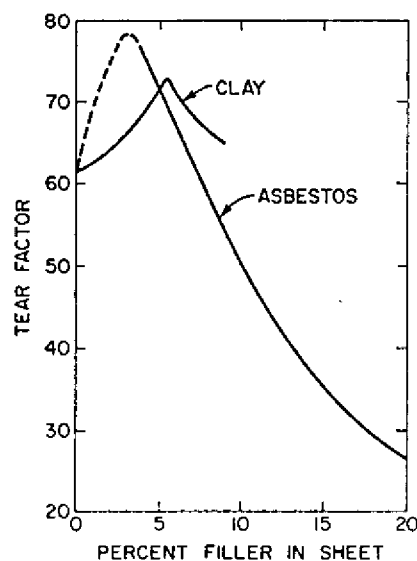
Fig. 9. Tear factor versus filler content
