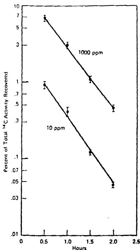
FIGURE 6. Expired vinyl chloride expressed as percentage of the recovered radioactivity vs. time following a 6-hr. exposure to 10 and 1000 ppm VC. Each point represents the mean \pm standard error of the mean of four rats. The curves were fit by linear regression analysis.
