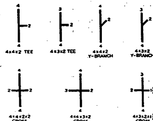
Fig. 1 . . . . Description of Tees and Laterals (ASA B16.3-1951)
