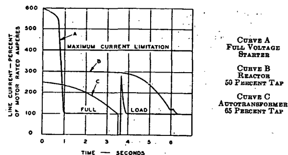
FIG. 5. STARTERS FOR MAXIMUM CURRENT LIMITATIONS
