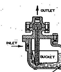
FIG. 26. UPRIGHT BUCKET TRAP
