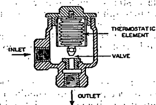
FIG. 23. THERMOSTATIC TRAP BELLOWS TYPE
