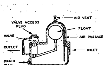
FIG. 21. SINGLE PORT FLOAT TRAP
