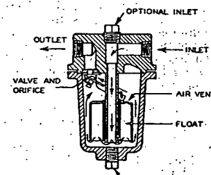
FIG. 28. INVERTED BUCKET TRAP WITH CENTRAL GUIDE
