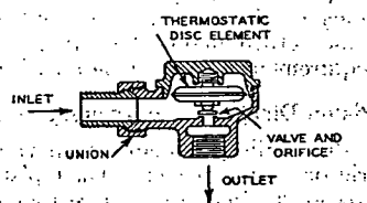
FIG. 24. THERMOSTATIC TRAP DISC TYPE
