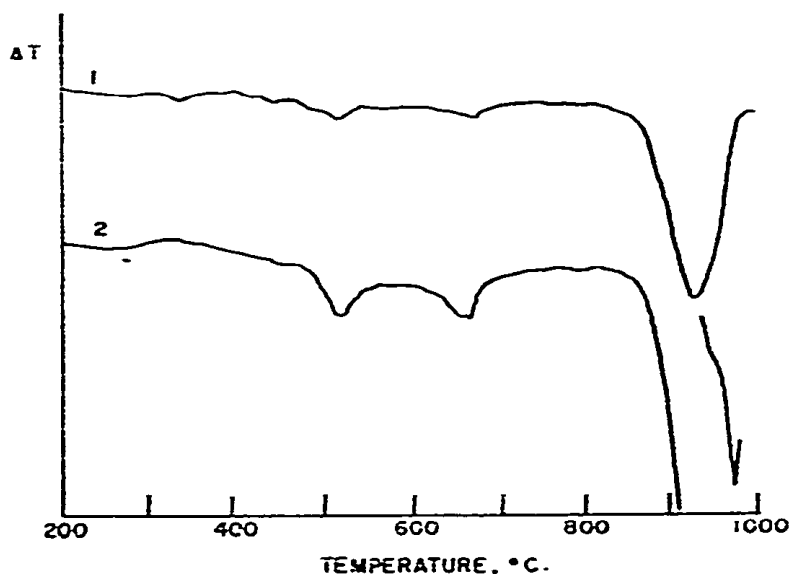
Fig. 1. DTA curves for talc run under normal (1) and more sensitive (2) conditions.
