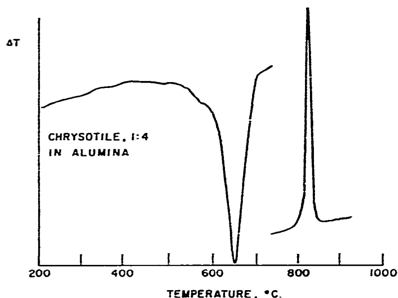
Fig. 3. DTA curve for chrysotile asbestos.
