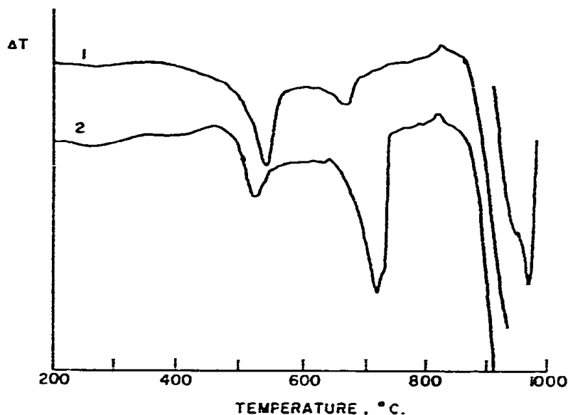
Fig. 2. DTA curves showing the effect of adding 1% magnesite (1) and 2% dolomite (2) to talc.
