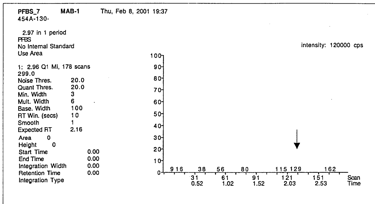
Figure 5. A representative ion chromatogram of a matrix blank sample (454A-130-MAB-1). The arrow indicates the retention time of PFBS.
