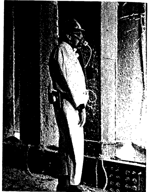
Figure 17. Because the spray applicators are subjected to high concentrations of asbestos fibers, some type of air filtration or supplied air respirator is necessary. A prototype of the Burgess filtered air respirator.
