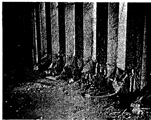
Figure 9. Custom-fabricated tarpaulins for building enclosure. Note tongues and tie-downs to prevent materials from dropping along the side of the building.
